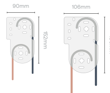
Figure 4 Diagram showing dual reverse bracket systems with window blind (red) and room blind (blue).
