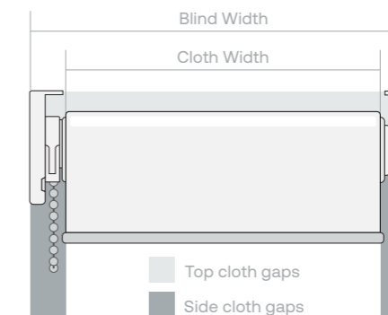
Figure 2 Diagram showing the difference between the overall blind width (outside of bracket to outside of bracket) and the cloth width. Applicable for both single and dual roller blinds.
