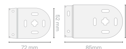
Figure 1 Diagram showing single roller blind bracket projections in a face fit position.
